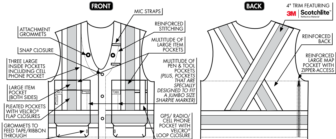
Two Inner Cell Phone/ Accessory Pockets with VELCRO® Loop Closures
